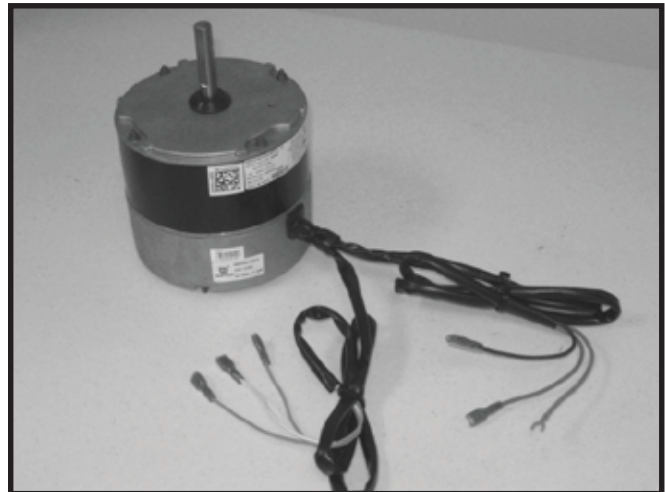
Figure 2. Replacement Motor (P/N's 1006722 or 1006723)
