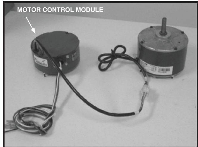
Figure 1. Original Motor With a separate control module (P/N's 622442 or 622468)
