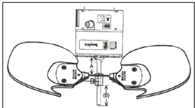
Figure 3. Fan Blade Position (Only for motor replacement with a separate control module)
